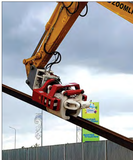
Handling/pithing/ driving/extracting (H - Beams)
