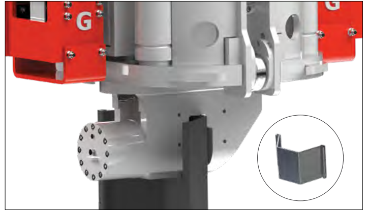
Handling/pithing/driving/extracting (Sheet Piles)
